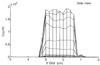
Figure 4.22 End and side views of the monostatic acoustic pulse for 5.2 MHz and wire of radius 50 microns.
